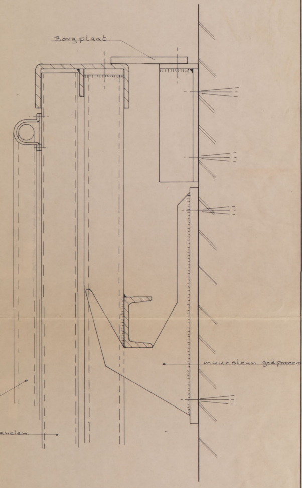
Detail A
